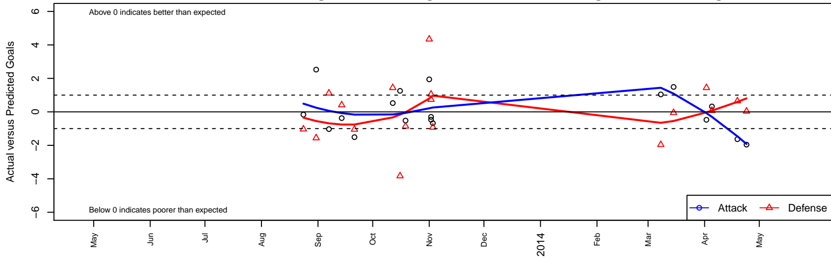
Meridian United FC Brazil G01 Dots are actual minus expected GF (blue circles) and GA (red triangles). Blue line is smoothed change in attack strength. Red is smoothed change in defense strength.
